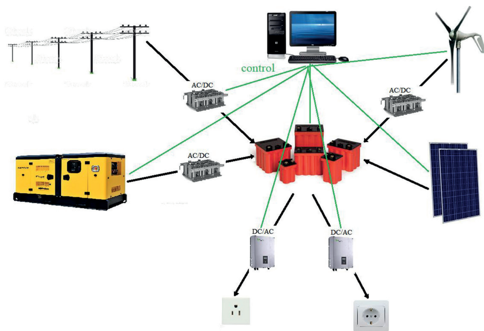
Figure 5. A possible “full-scale” smart grid structure.
